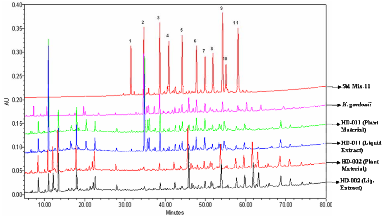
Figure 4. HPLC profiles of Hoodia gordonii demonstrating presence of 11 diagnostic oxypreganane glycosides.
